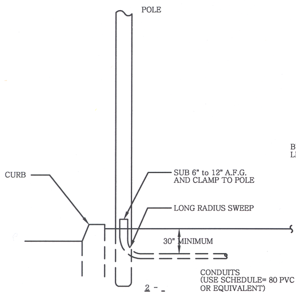
CONDUIT FEED FROM POLE
